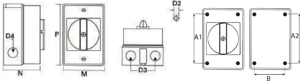
Dimension IP65 plastic box
